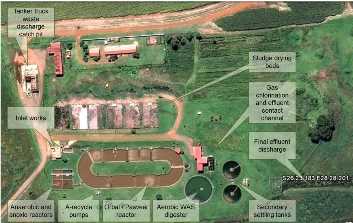
FIGURE 1: PLANT LAYOUT
